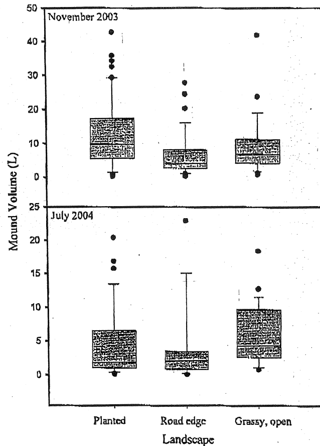
Fig. 2. Box-and-whisker plots of imported fire ant mound sizes (volume in L) in three landscape types within south-central TN ball-and-burlap nurseries.
